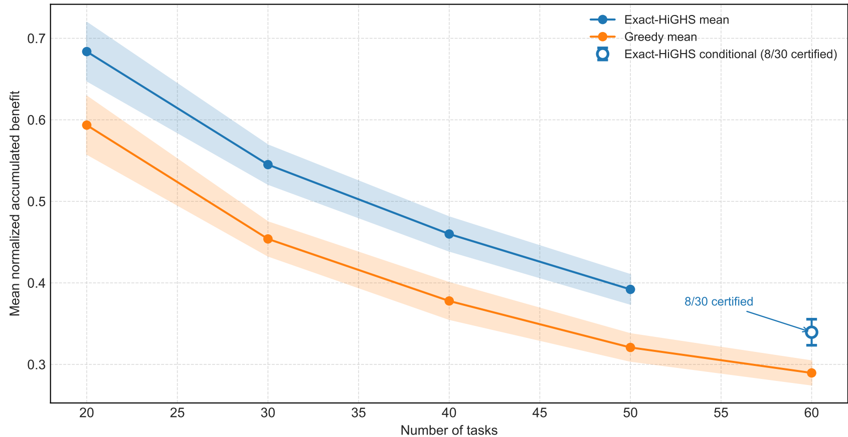
Experiment B: normalized benefit across task counts
